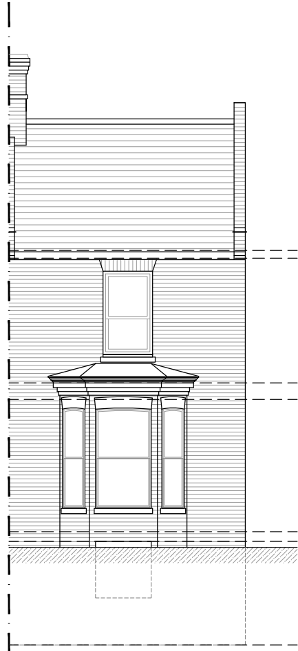
Front (North-West Facing) Elevation 1:100
